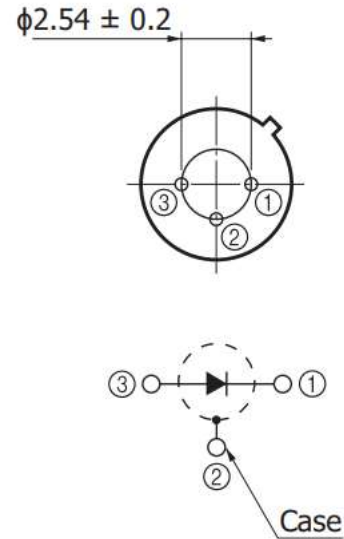
Bottom view
